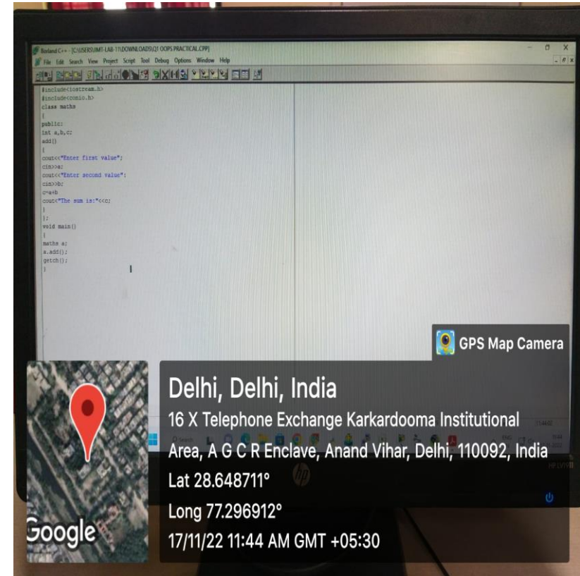
Borland C++
