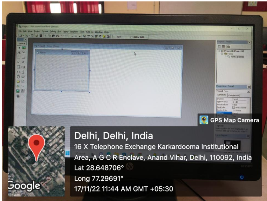
Visual Basic 6.0
