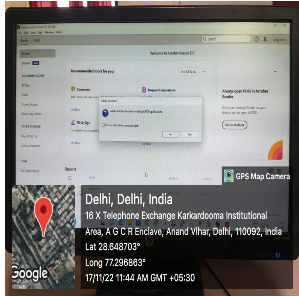
Adobe Reader
