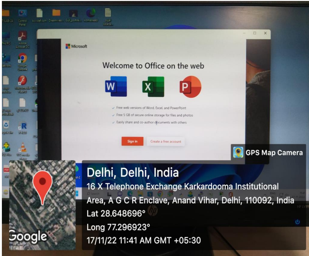
Microsoft office – 2007
